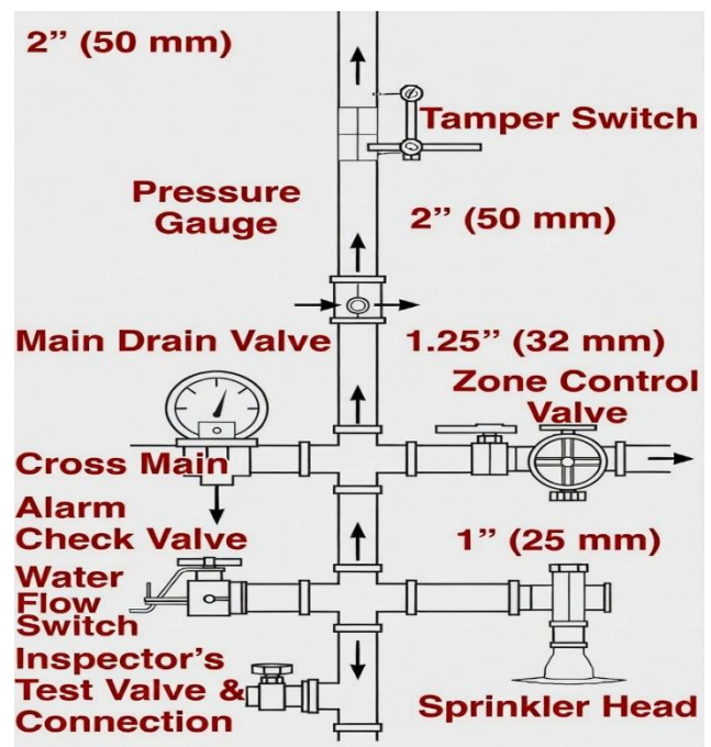
Fig.8: Sprinkler pipe, valves & accessories
